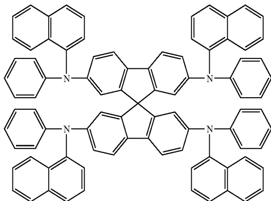
spiro-NPB
