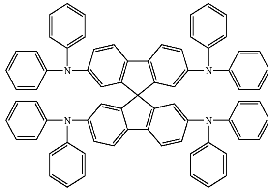
spiro-TAD
