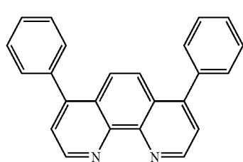
Bphen
