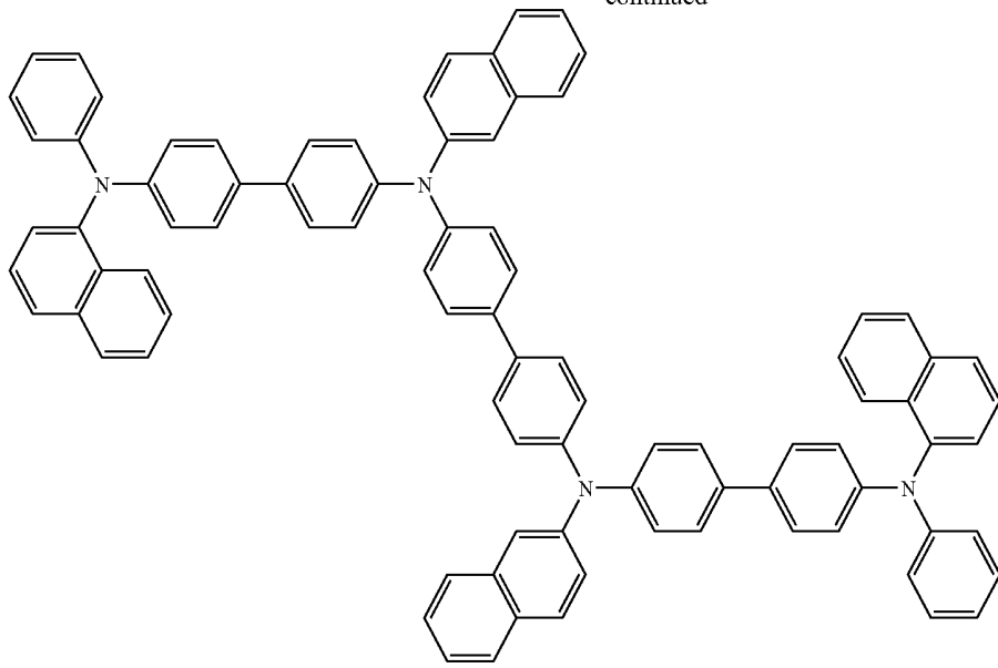
DNPD
