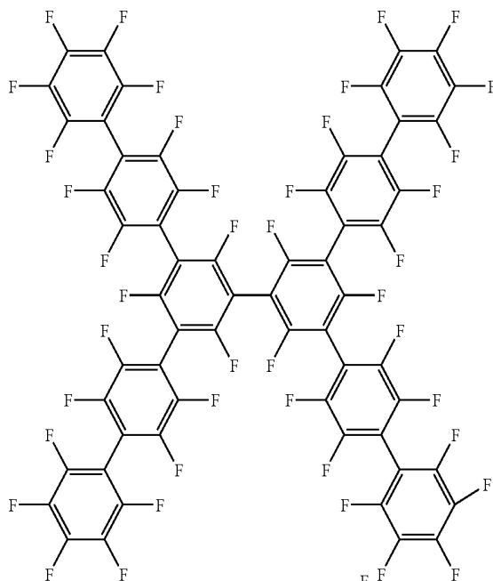
CF-X
