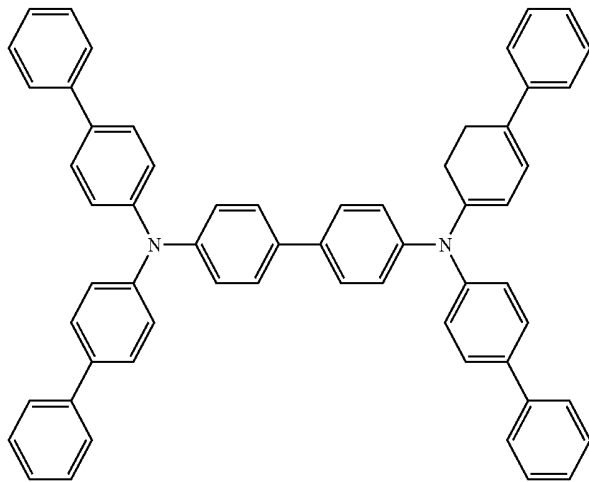
TBPB
