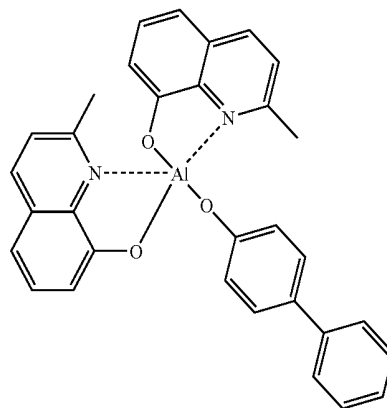
BA1q
